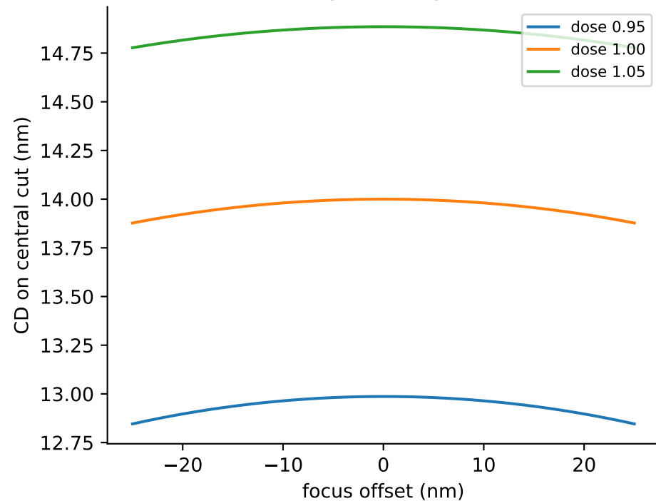
Teaching Bossung curves
